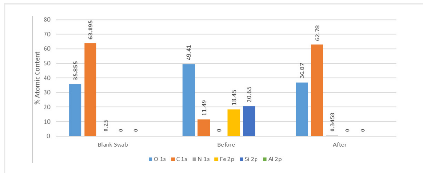
Figure 3: XPS analysis of railhead swabs, left – blank swab, centre – rail before treatment, right – after treatment.
