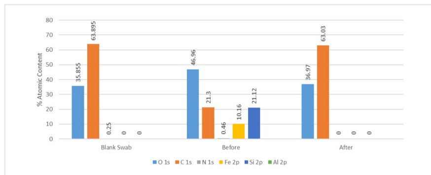
Figure 4: XPS analysis of railhead swabs; left – blank swab, centre – rail before treatment, right – after treatment.
