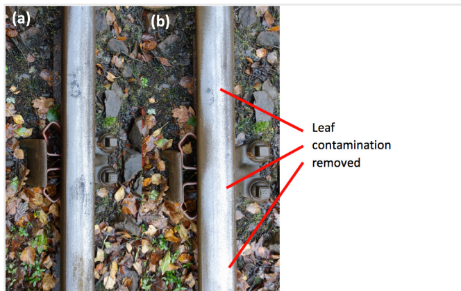
Image 6: Level 1 leaf contamination present on the railhead before treatment (a), leaf contamination removed (b)
