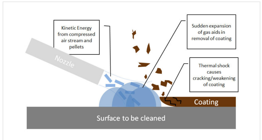
Figure 1: The three mechanisms of dry ice cleaning.
