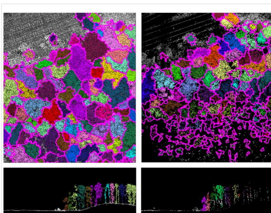
Figure 4: Left - FLI-MAP plan and elevation; Right - RILA plan and elevation.
