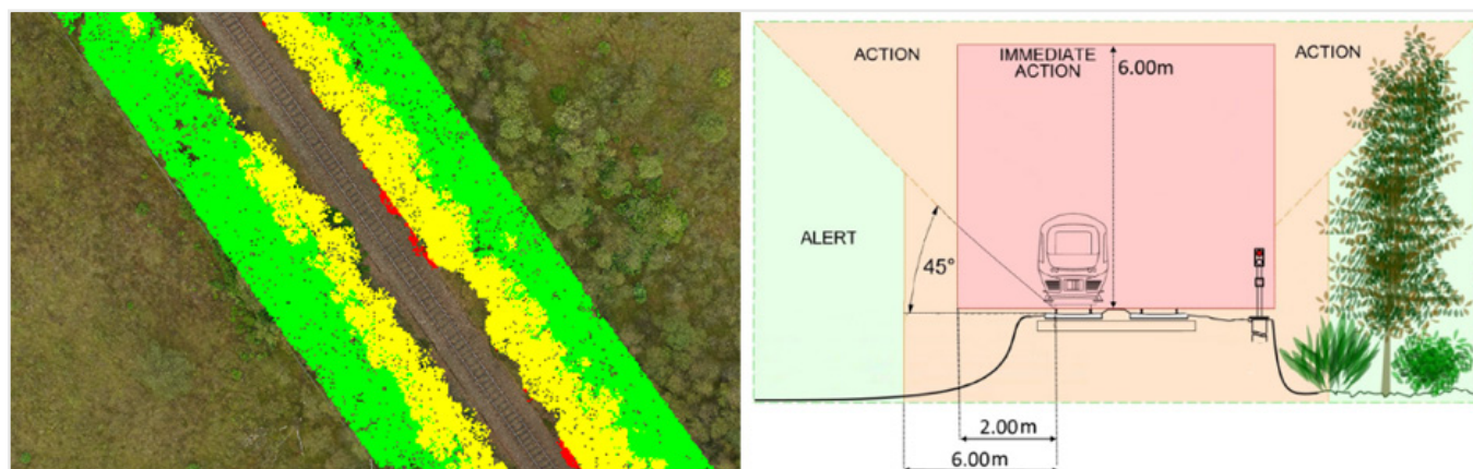
Figure 2: Left - Example risk map showing vegetation in the immediate action zone (in red), in the action zone (yellow), and in the alert zone (green). Right - Intervention zone profile used.
