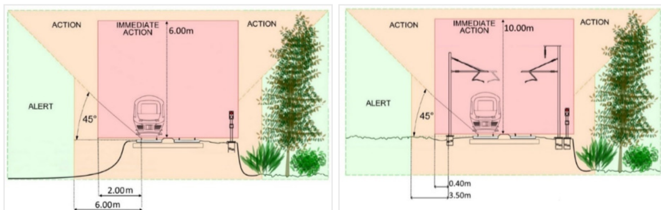
Figure 1: Left - Non-electrified intervention zones; Right - electrified intervention zones as detailed in NR/L2/OTR/5201_01, issue 3.
