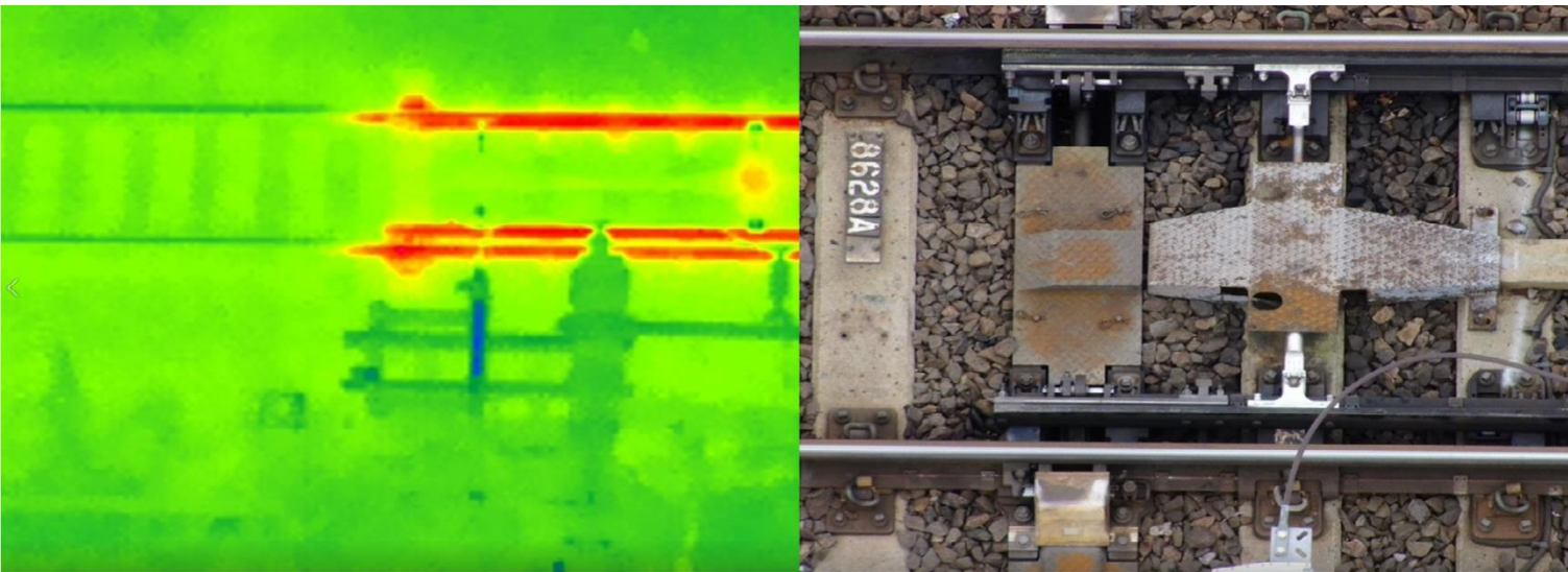
Points Heating C2 Inspection with a Thermal image Overlay
